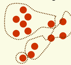
bad clustering
