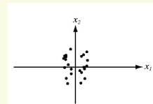
after normalization
