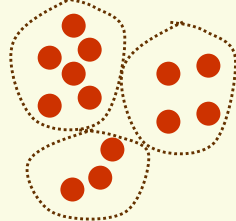
good clustering
