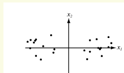
before normalization
