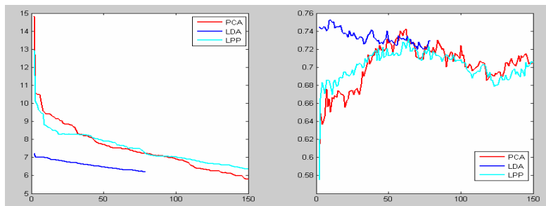
Fig.4 Left side shows the age error in a 5-fold cross variation set, and right side shows the age classification precision in test set. The x-coordinate of both figures indicates the reduced dimension, and from left to right, the y-coordinate represents mean age error and classification precision respectively.
