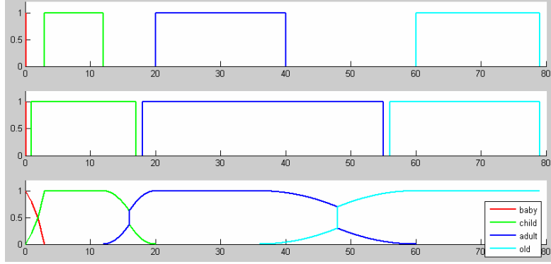
Fig.2. Three kinds of fuzzy age membership functions: on the top, only non-vague ages are assigned to a certain age group, while in the middle, all ages are belonging to exactly one group, at the bottom is the more natural one being fuzzy because it takes into account of the age ambiguity.
