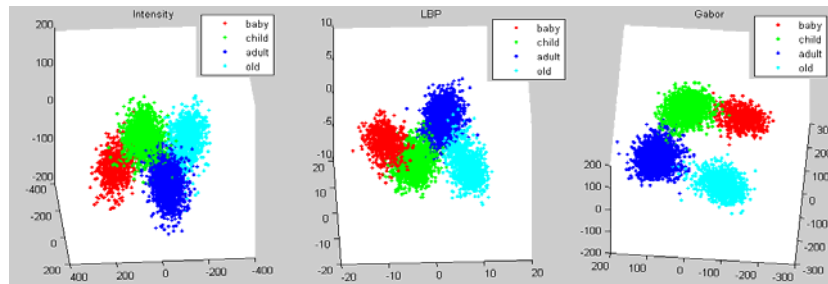
Fig.3. The training data visualization in discriminative feature space (left for intensity feature, middle for LBP feature, right for Gabor feature)
