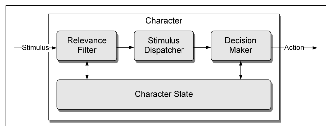
Figure 4. Psychosocial Character Architecture
