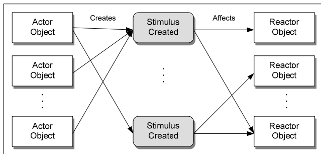
Figure 2. A Generalized Stimulus-Response System
