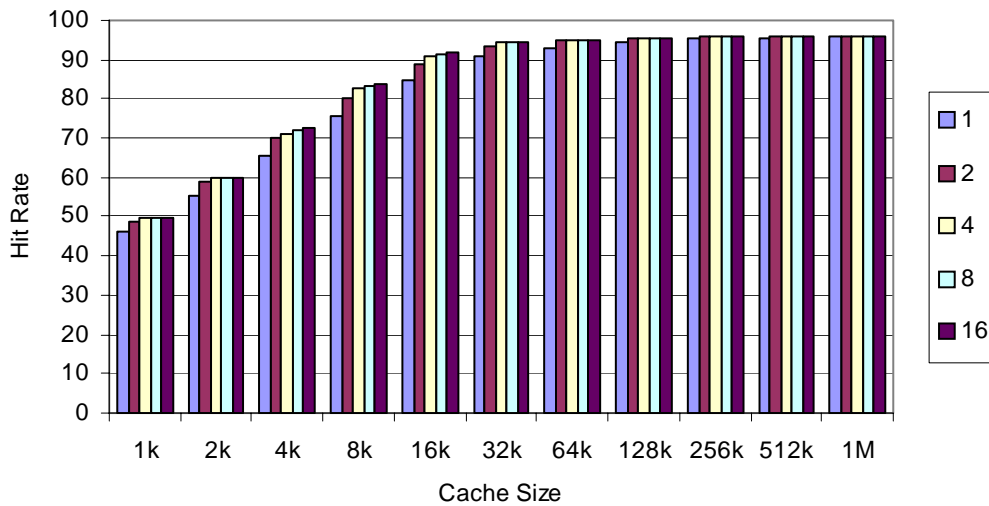
Figure 2. Varying Associativity over Cache Size
