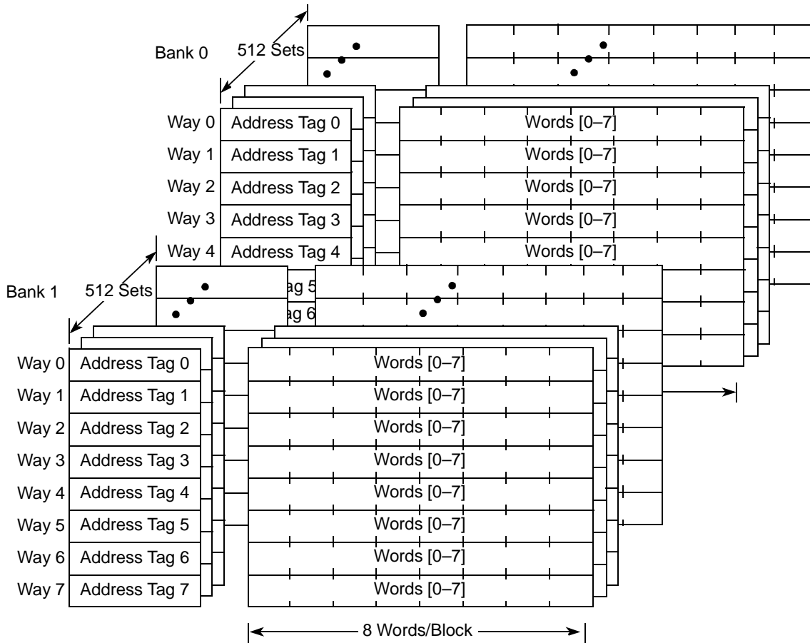
Figure 15. L2 Cache Organization
