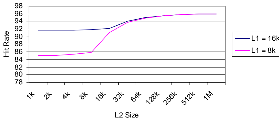
Figure 8. Total Hits (L1 and L2) for 8 Kbyte and 16 Kbyte L1
