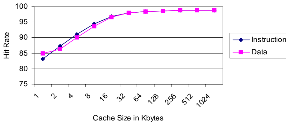
Figure 9. Instruction versus Data Hits for L1 Cache
