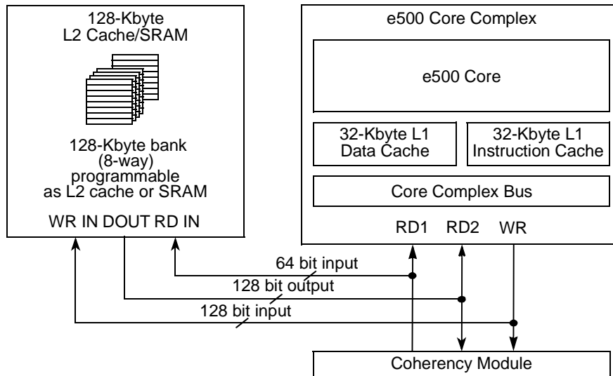
Figure 13. e500 Core and Caches
