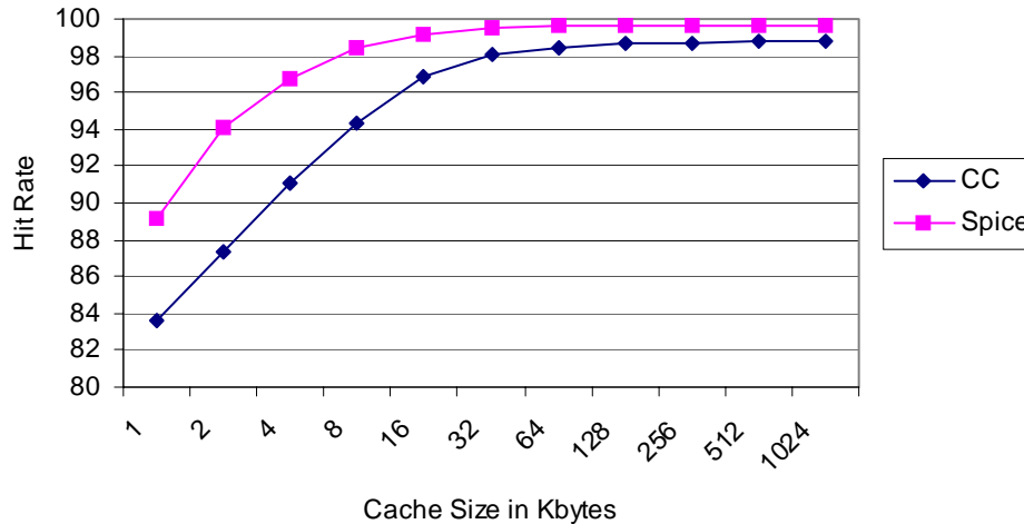
Figure 5. L1 Cache Hits
