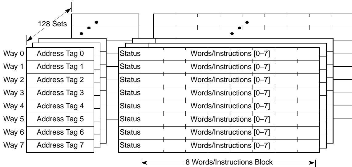
Figure 14. L1 Cache Organization
