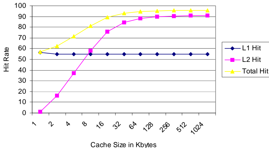
Figure 6. Hit Rates for Increasing L2 Cache Size, with 1 Kbyte L1
