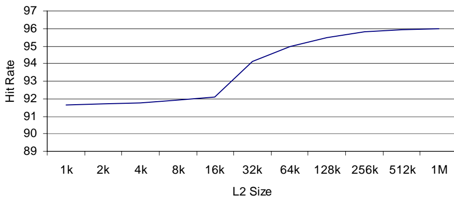
Figure 4. 16 Kbyte L1 versus L2
