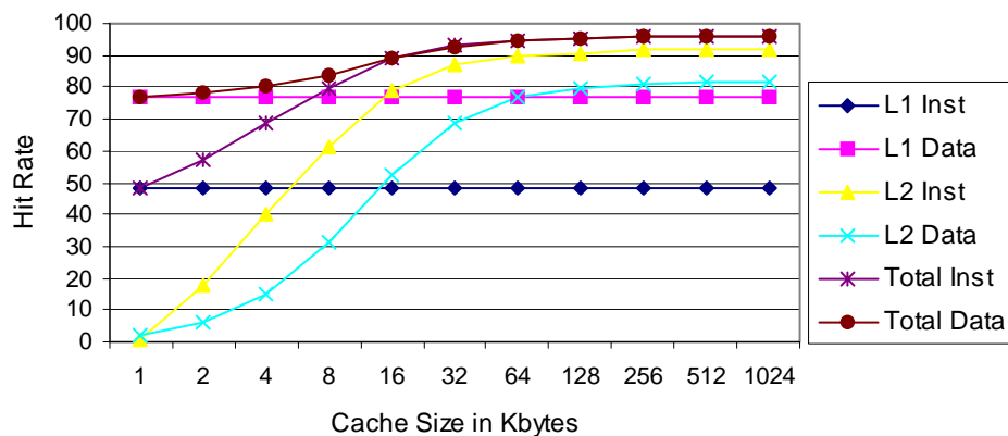
Figure 10. L2 Instruction versus Data Cache Hits (Varying L2 size)
