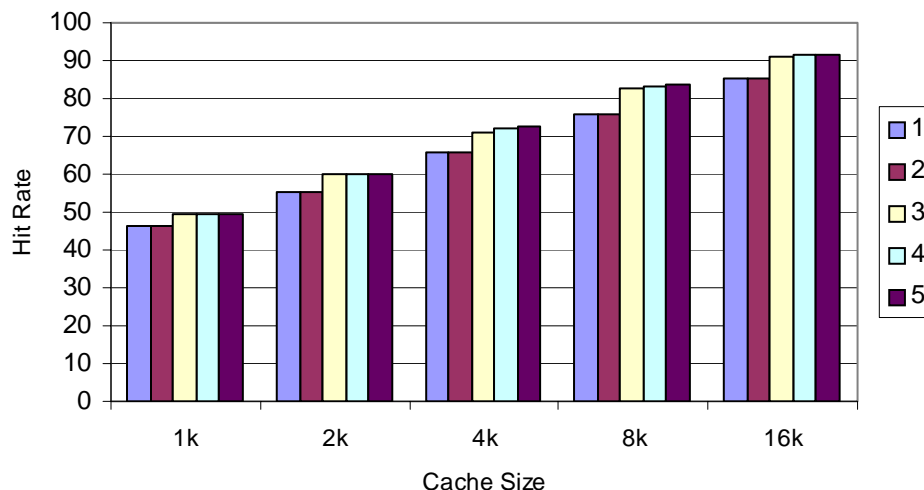
Figure 3. Zooming in on Associativity versus Cache Size
