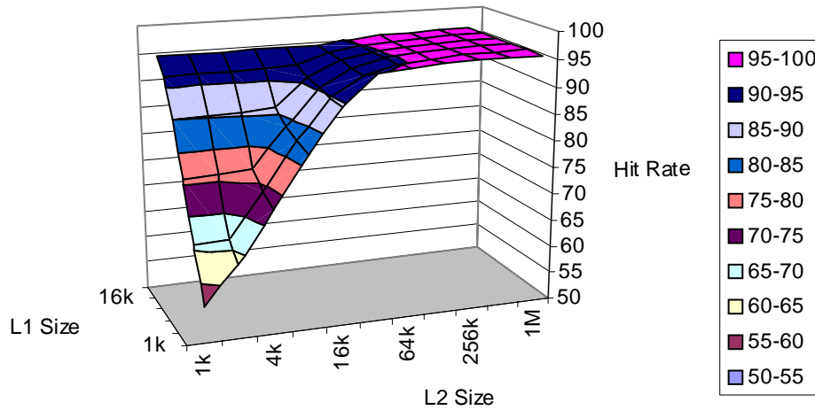
Figure 7. Hit Rates for Changing L1 and L2 Size
