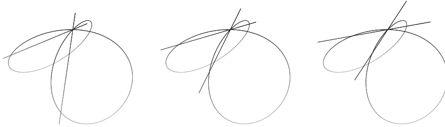
Fig. 3. Secants along \mathbf{V}(x^2 + y^2 + z^2 - 1) \cap \mathbf{V}(x^2 - y^2 - z(z - 1)) limiting to (0, 0, 1) .
