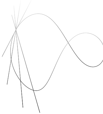
Fig. 2. Limiting secants along \mathbf{V}(x^2 + y^2 + z^2 - 1, x^2 - y^2 - z) .
