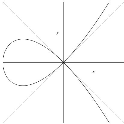
Fig. 1. This figure displays the typical “fish” curve, which is a planar curve given by h = y^2 - x^2(x + 1) \in \mathbb{Q}[x, y] . Clearly, two tangent lines are needed to form a “linear approximation” of the curve at the origin. Elementary calculations show these two lines actually form the tangent cone of the fish curve at the origin.
