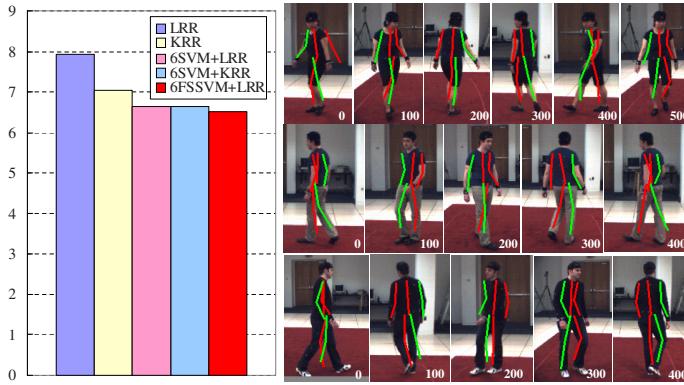
Fig. 6. Results of pose estimation on HumanEva-I dataset. The left bar graph shows pose prediction errors with respect to different regression methods. The right images show samples of predicted poses for 3 subjects drawn in the red and green (right arm and leg) line segments. (The head top joint (headDistal) is not used because of error in the dataset.)
