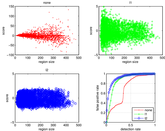
Figure 2. Normalization and bias. A linear SVM is trained to discriminate image regions R that do and do not portray a car (for VOC 07 training and testing). The figure compares using un-normalized, l^1 -normalized, and l^2 -normalized histograms. The first three panels are scatter plots of the SVM score C(h^R) (for some positive and negative test regions) and the square root of the region area. The un-normalized scores reward large regions, the l^1 -normalized scores small regions, and the l^2 -normalized scores are essentially unbiased. The last panel shows the ROC curve for the three classifiers, illustrating that l^2 normalization performs best.
