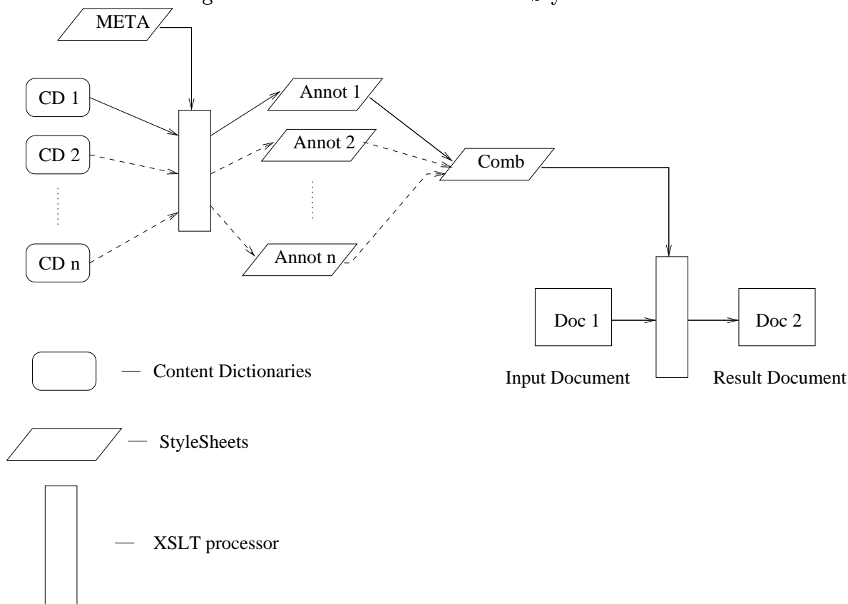
Figure 1: Automatic Production of Stylesheets
