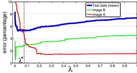
Figure 6. Image segmentation - error statistics. The number of misclassified pixels (error) varies with respect to \lambda . The optimal \lambda does also vary considerably among test images (images A and B are shown in [24]).
