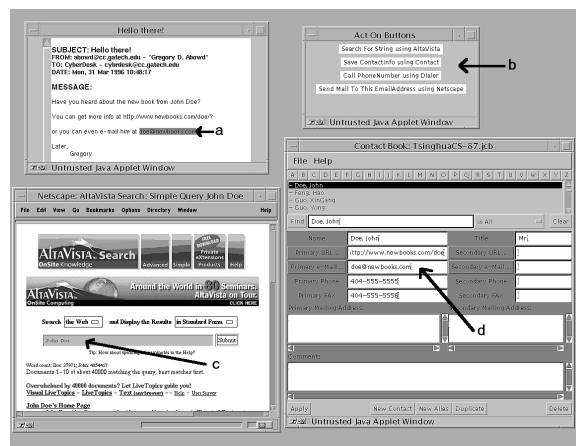
Figure 2: An annotated scenario of usage for the CyberDesk system.
