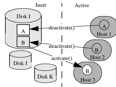
FIGURE 4. A sample subset of Legion comprising three disks (I, J, and K) and three hosts (1, 2, and 3). Objects A and B are moved between Active and Inert states. Object A has been deactivated into an Object Persistent Representation on Disk I, and B has been migrated from Host 2 to Host 3 through Disk I
