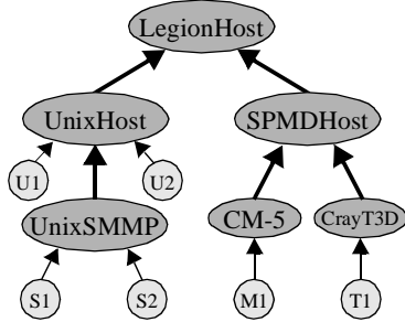
FIGURE 1. The Legion class LegionHost is the root of all classes whose instances are Legion Hosts. In this figure, UnixHost and SPMDHost are derived directly from LegionHost. UnixSMMP is derived from UnixHost, and CM-5 and CrayT3D are derived from SPMDHost. The figure shows six different Legion Hosts: two instances of both UnixHost and UnixSMMP, and one instance of both CM-5 and CrayT3D.
