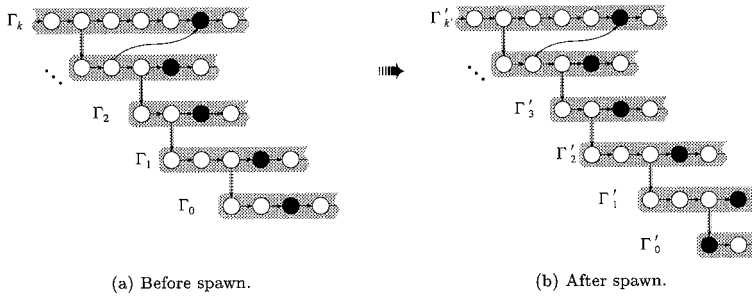
FIG. 4. The ready deque of a processor before and after the thread \Gamma_0 that it is working on spawns a child. (Note that the threads \Gamma_0 and \Gamma'_0 are not actually in the deque; they are the threads being worked on before and after the spawn.)
